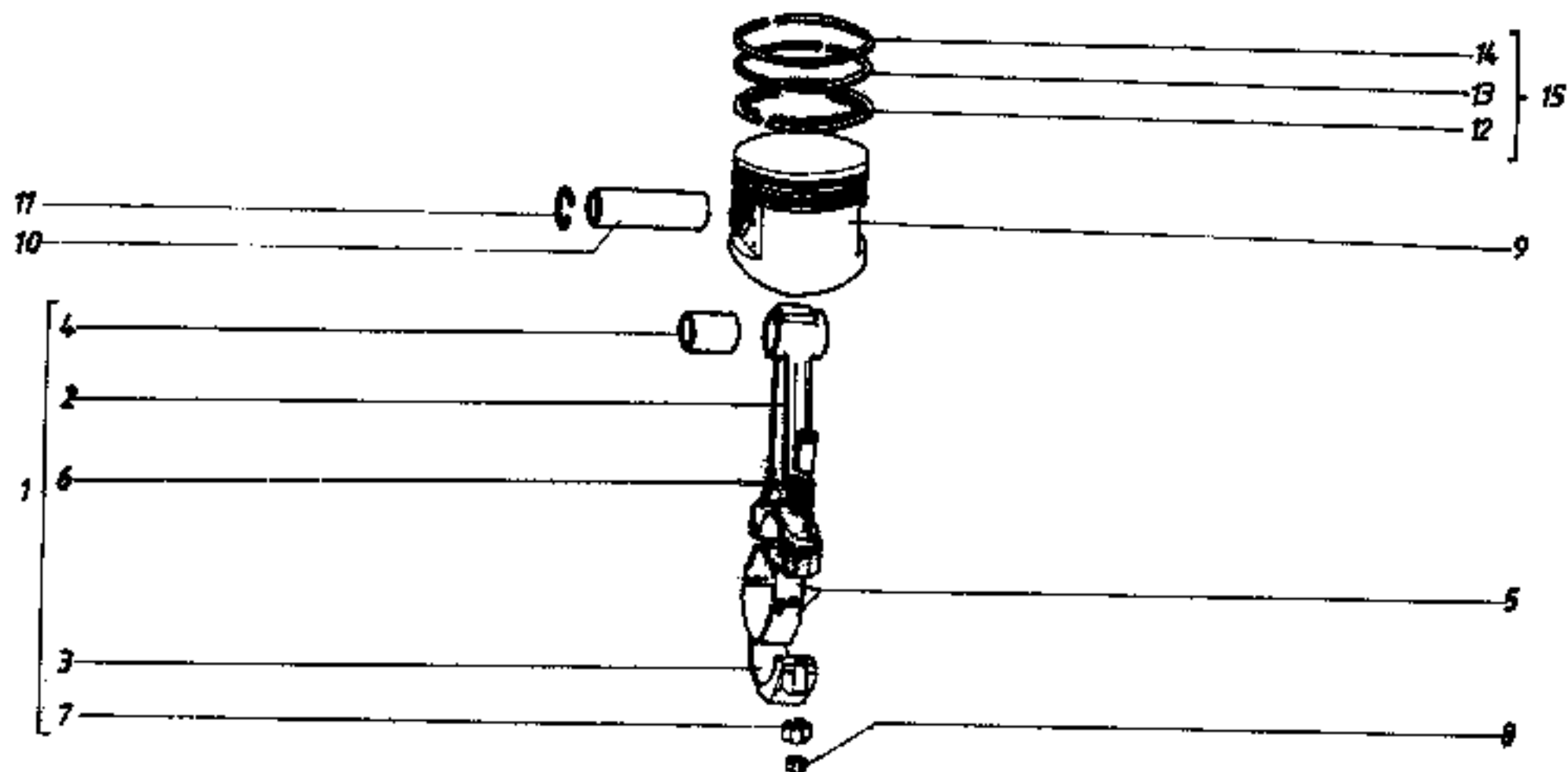
Ensemble Bielle - Piston
